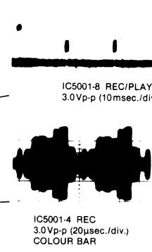
IC5001-4 REC 3.0Vp-p (20uSec/div) COLOUR BAR
